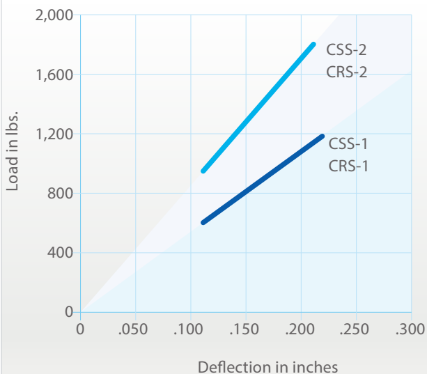
Load versus Deflection Chart
