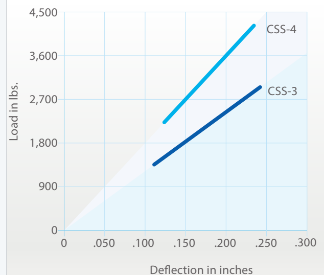
Load versus Deflection Chart
